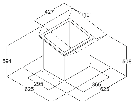
Kit tetto piano Flat roof kit
