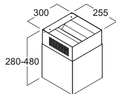
Chimenea filtrante Filtering chimney
