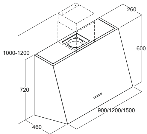
Camino aspirante Suction chimney
